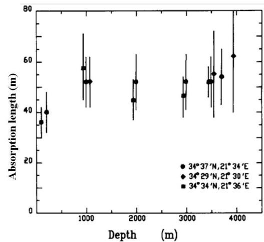
Figure 6-3: Absorption length versus depth at 460 nm wavelength in the Pylos area.
