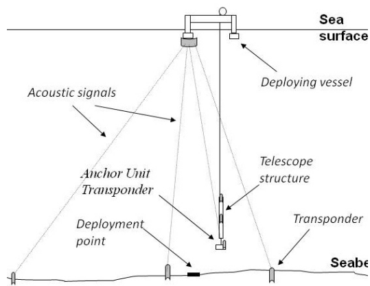
Figure 7-23: Components of the sea bottom positioning system
