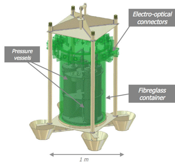
Figure 5-8: The junction box of the NEMO Phase-1 project.
