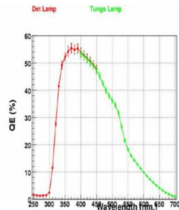
Figure 7-10: Measured photocathode quantum efficiency for the Photonis special Bi-alkali photocathode.
