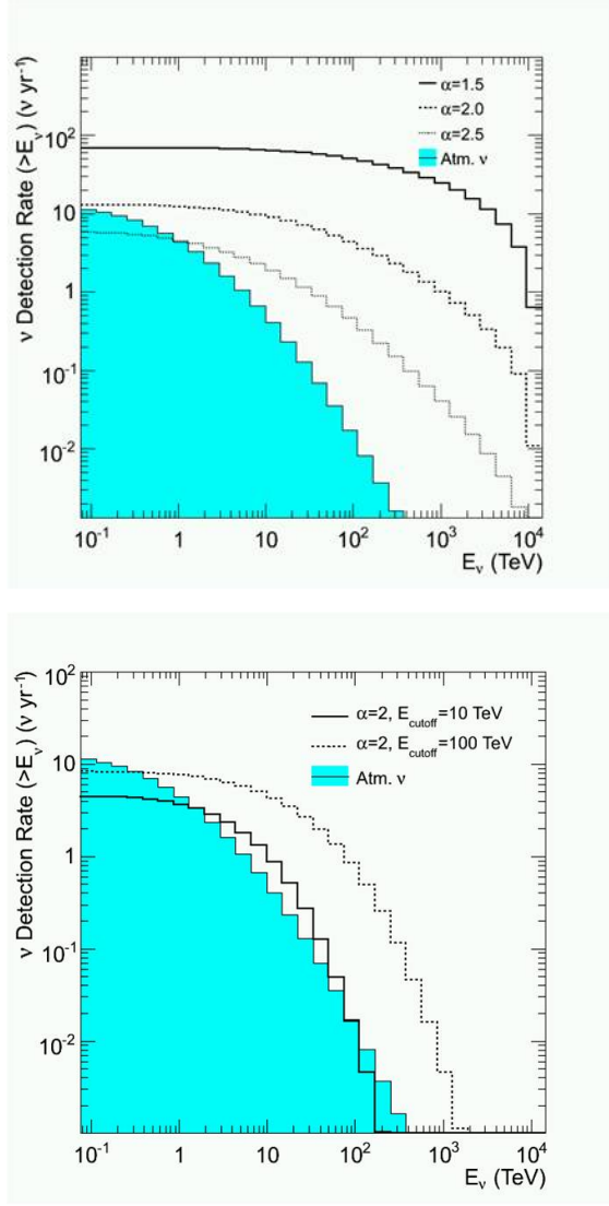
Figure 2-2: The total rates above each energy detected by KM3NeT for the spectral indices \alpha=1.5 , 2, 2.5 and no energy cut-off (upper), and for a single spectral index of \alpha=2 and different cut-off energies E_0=10 , 100 TeV (lower).
