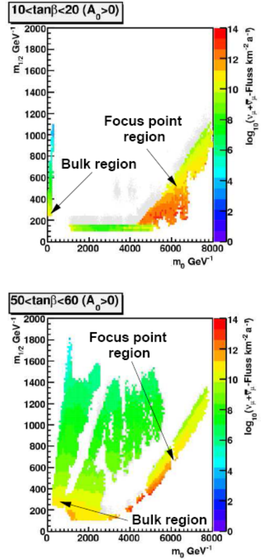
Figure 2-7: Neutrino flux on the Earth as a function of mSUGRA parameters.
