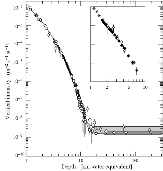
Figure 1-3: Vertical muon intensity versus depth (1 km water equivalent = 10^5 \text{ g cm}^{-2} of standard rock). The experimental data are from: \diamond : the compilations of Croux (12), \square : Baksan (13), \circ : LVD (14), \bullet : MACRO (3), \blacksquare : Frejus (15), and \triangle : SNO (16). The shaded area at large depths represents neutrino-induced muons of energy above 2 GeV. The upper line is for horizontal neutrino-induced muons, the lower one for vertically upward muons.
